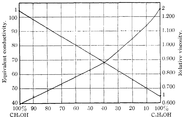
Curve 1.—Composition—conductivity. Curve 2.—Composition—viscosity.
